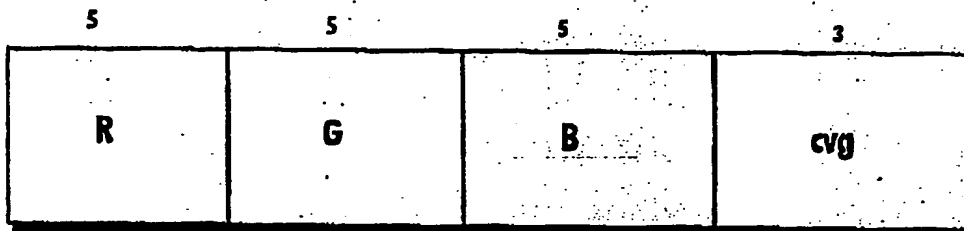
Fig. 32 COLOR PIXEL FORMAT
